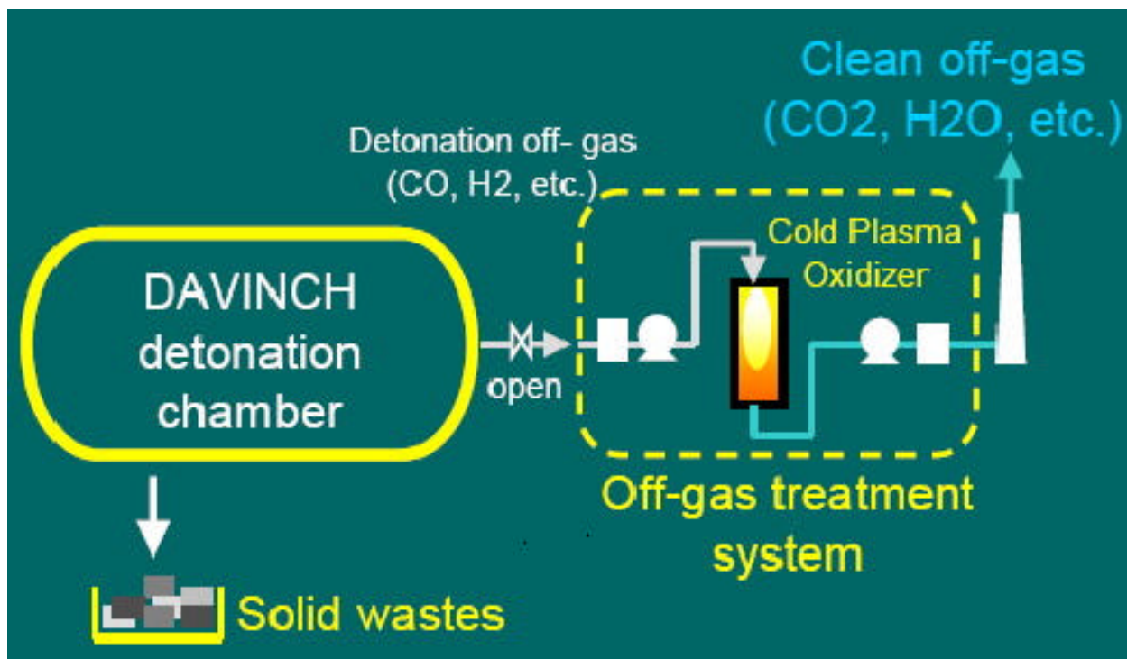
Fig. 4. Principle of the technology [4]
