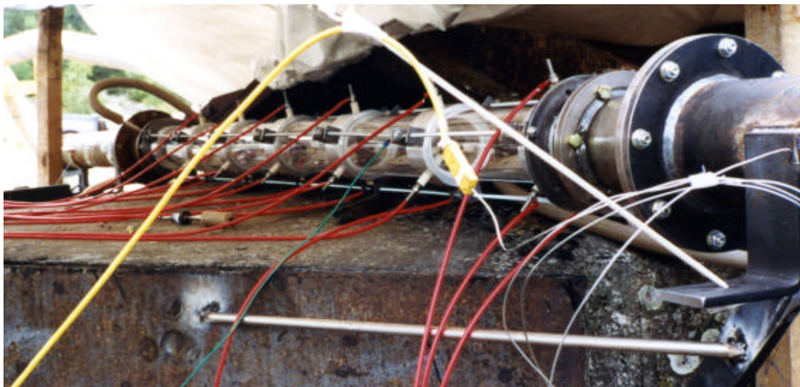
Fig. 3. GlidArc reactor for flue gas cleanup
