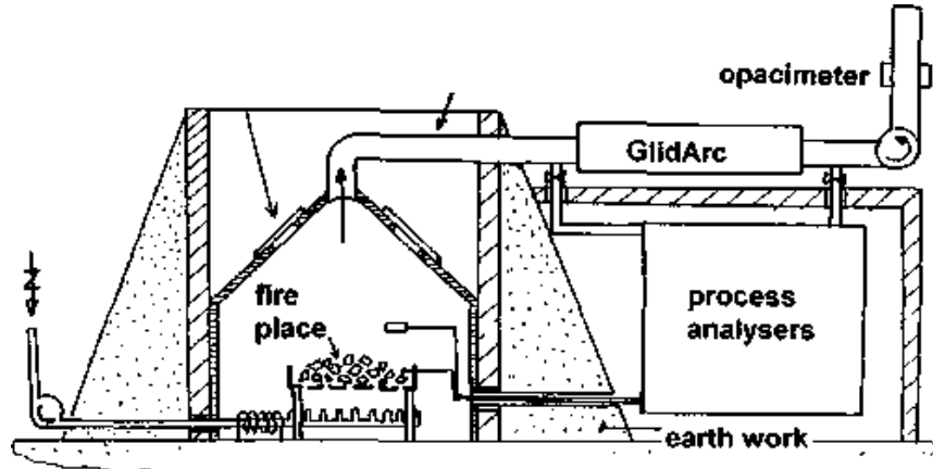
Fig. 2. Pilot plant for TNT burning and Flue Gas cleanup
